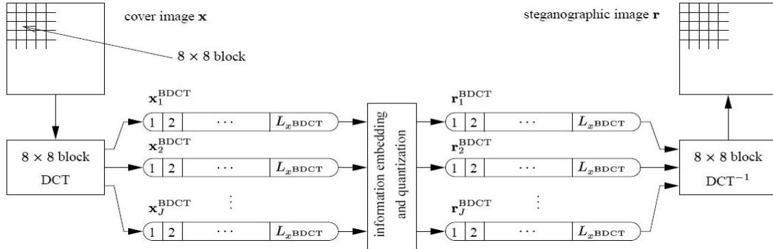
Figure 7. Image Steganography using the 8 x 8 Block DCT (BDCT).
