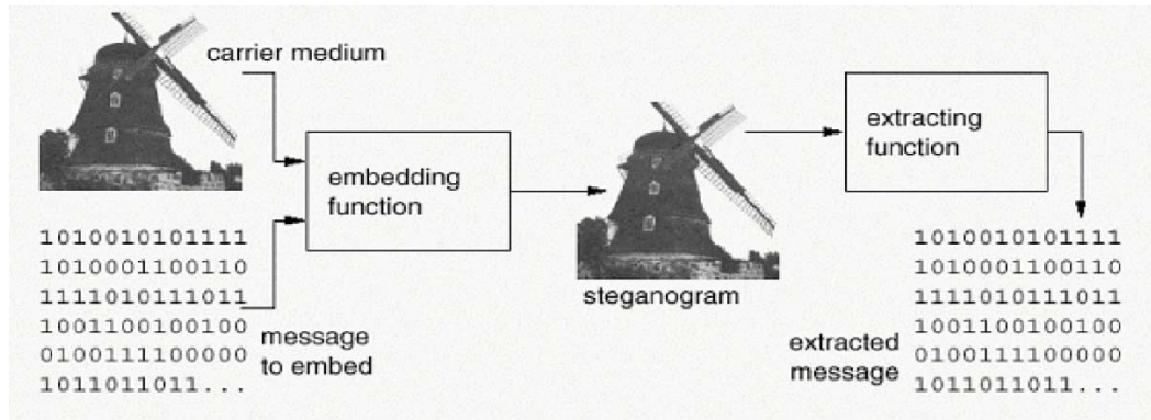
Figure 6. LSB for Image-Steganography.
