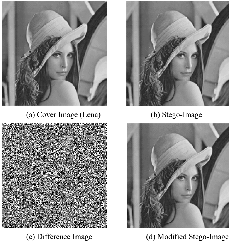
Figure 10. Hiding Plaintext Message into Lena Image (Steganography).
