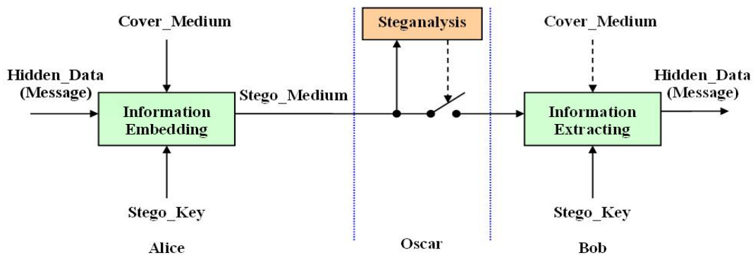
Figure 2. Dataflow for Information Hiding with an Adversary (Steganography).
