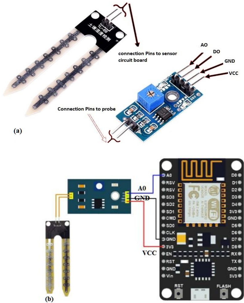
Figure3: (a)connecting of pin probe to sensor circuit board , (b) connecting of pins to ESP8266 board
