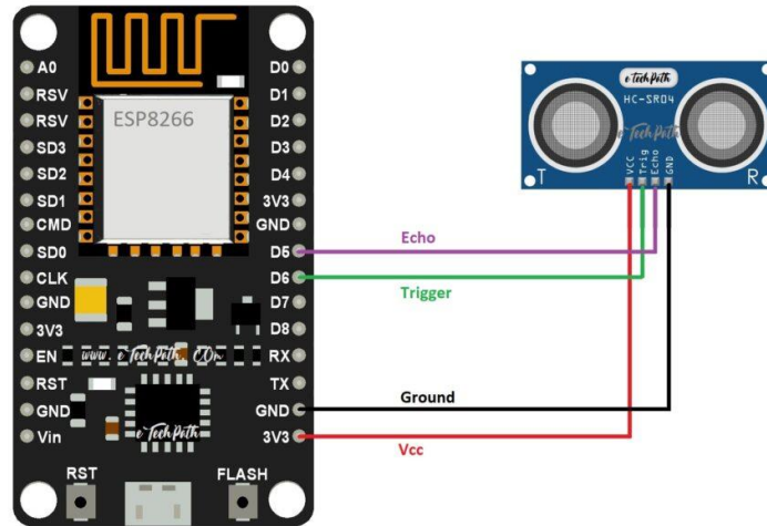
Figure 9: connecting of HC-SR04 Module sensor pin to ESP8266 board
