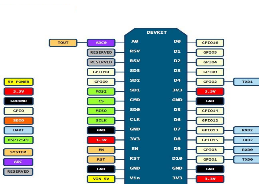
Figure2: Pin assignment of ESP8266 board.
